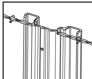
Barb wire can be twiched to the top of the post if required
