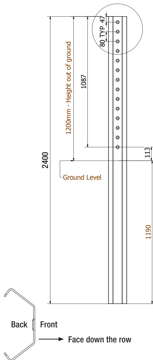
2400mm - 14 holes
