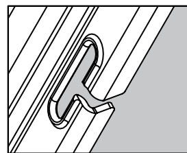
Rounded wire holes to reduce abrasion
